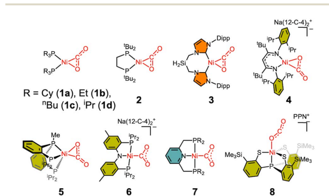
Scheme 1 Structurally characterized Ni-CO 2 adducts.
