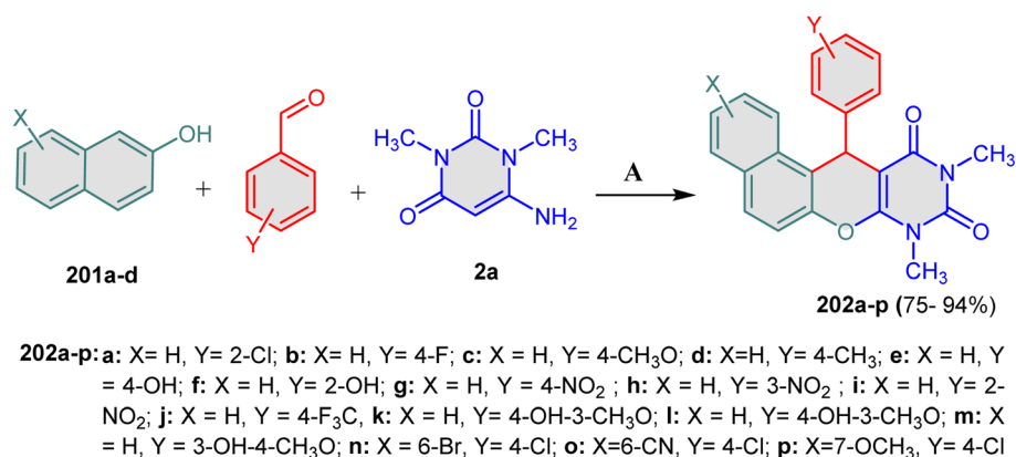
Scheme 75 Formation of chromeno[2,3- d ]pyrimidines 202a–p . Reagents and conditions: A = ChCl: \alpha -CAA (1 : 1), 90 °C, 2 h.
