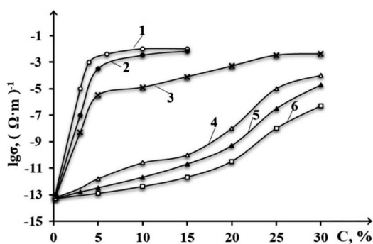
Fig. 13 The influence of graphite concentration on the electrical conductivity of compatibilized HDPE + EPDM polymer blends: (1) – HDPE; (2) – HDPE + 10 wt% EPDM; (3) – HDPE + 30 wt% EPDM; (4) – HDPE + 40 wt% EPDM; (5) – HDPE + 50 wt% EPDM; (6) – HDPE + 70 wt% EPDM. 185
