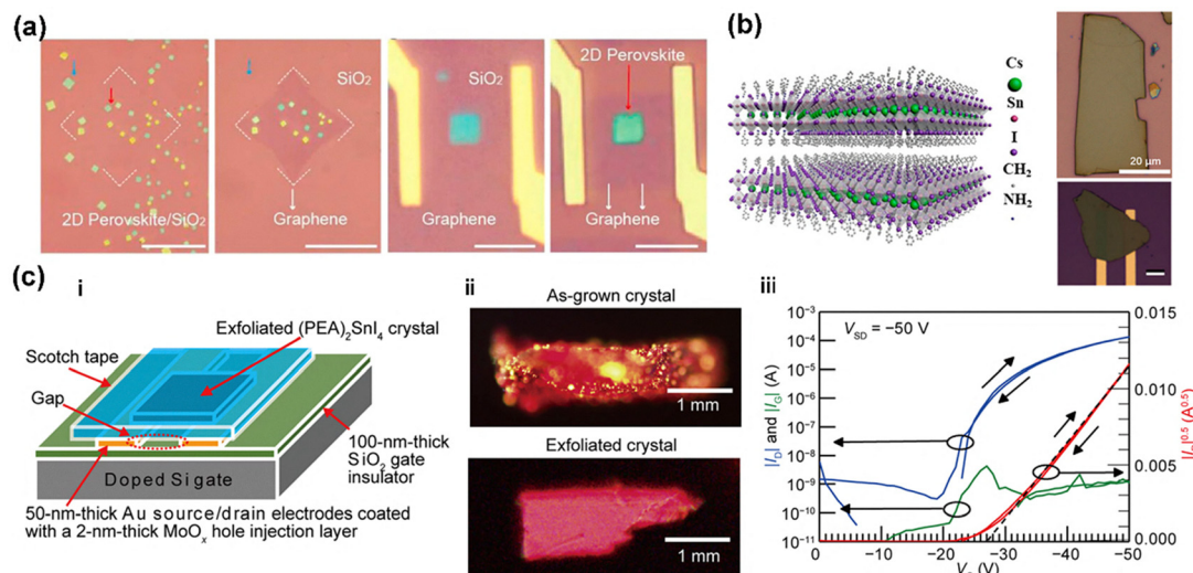
Fig. 6 (a) Optical images of the growth process of 2D (C_4H_9NH_3)_2PbBr_4 crystals and the transfer process of a graphene protective layer and 2D (C_4H_9NH_3)_2PbBr_4 device with graphene electrodes. The scale bar of the first and the second are 50 \mu m , and the third and the four are 10 \mu m . 103 (b) Schematic illustration and optical image of the crystal structure of (PEA)_2CsSnI_7 perovskite and the optical image of the corresponding device. 8 (c) (i) Schematic architecture of a (PEA)_2SnI_4 crystal FET. (ii) Optical microscopy images of the as-grown and exfoliated (PEA)_2SnI_4 crystals. (iii) Transfer curves were obtained in nitrogen. 104 Figures reproduced with permission from: (a) ref. 103. Copyright 2016, (b) ref. 8. Copyright 2019, American Chemical Society; (c) ref. 104.
