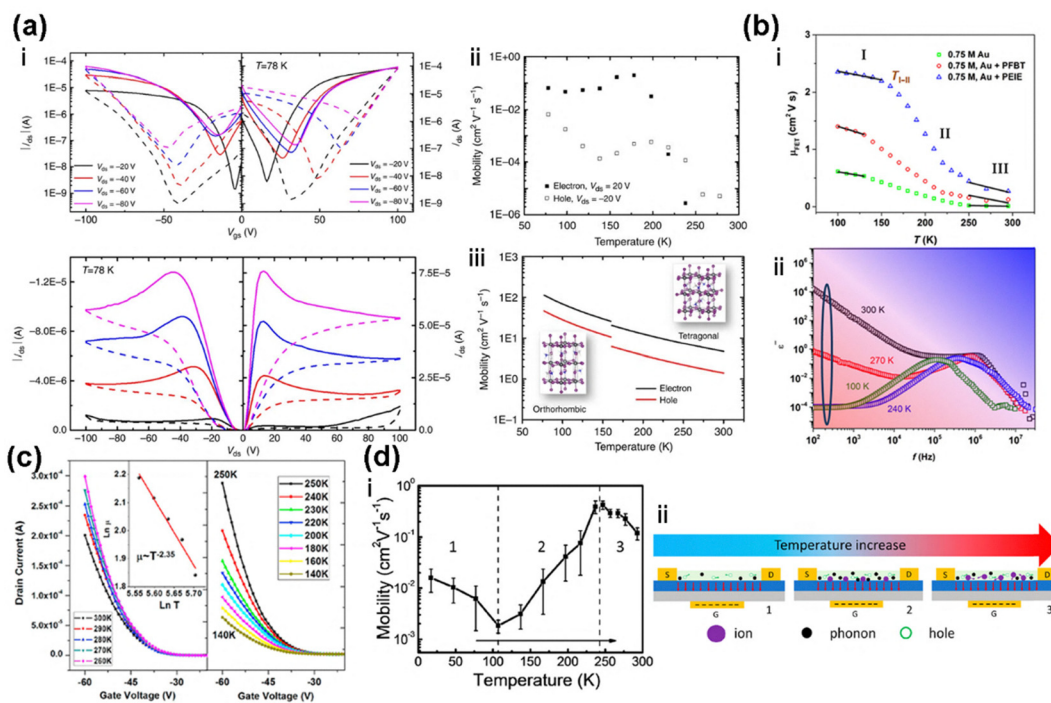
Fig. 4 (a) (i) Ambipolar transfer (top) and output (bottom) characteristics of CH 3 NH 3 PbI 3 FETs obtained at 78 K. Solid and dashed curves are measured with forward and backward sweeping, respectively. (ii) Temperature dependence of field-effect electron and hole mobilities. (iii) Calculated temperature dependence of hole (red curves) and electron (black curves) mobility in tetragonal ( T = 300 to 160 K) and orthorhombic ( T = 160 to 77 K) phases of CH 3 NH 3 PbI 3 . The crystal unit cells of the two phases are shown as insets. 46 (b) (i) The curves of \mu_{\text{FET}} - T with different interlayers at the S–D contacts depicting three different regimes of charge transport with a power law behavior: \mu \sim \mu_0 T^{-\gamma} . Region I: inorganic cage vibrational disorder ( \gamma \sim 0.2 to 0.4); region II: dominated by the polarization fluctuation of MA + ; region III: dominated by ion migration ( \gamma \sim 4.1 to 5.3). (ii) Corresponding dielectric loss measurement as a function of frequency and temperature. 79 (c) Temperature-dependent transfer curves of MAPbI 3 /C8BTBT hybrid FETs in the dark, the inset shows a band-like behavior in the relationship between mobility and temperature above 260 K. 33 (d) (i) Temperature dependence of the transistor mobility. (ii) Schematic diagram of the operating mechanism regarding the charge carrier transport. 39 Figures reproduced with permission from: (a) ref. 46. Copyright 2015, Springer Nature; (b) ref. 79. Copyright 2017; (c) ref. 33. Copyright 2016, Elsevier; (d) ref. 39. Copyright 2017, American Chemical Society.
