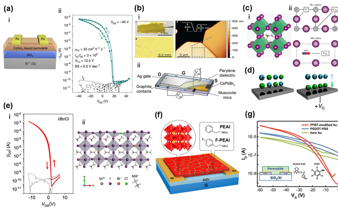
Fig. 3 (a) (i) BGTC TFT structure based on \text{CsSnI}_3 perovskite. (ii) Transfer characteristics of optimized \text{CsSnI}_3 ( \text{CsI}/\text{SnI}_2 = 1.25 ) perovskite channels processed from the Pb-substituted (10 mol%) precursor containing 7 mol% \text{SnF}_2 as additive. I_g in (ii) indicates the gate leakage current. 37 Reproduced from ref. 37 with permission from the Springer Nature. (b) (i) Optical photograph (1), optical microscopy image (2), and AFM topography image (3) of large-area epitaxial single-crystal \text{CsPbBr}_3 thin films. (ii) A sketch of the coplanar TCTG FET structure with large-area epitaxial single-crystal \text{CsPbBr}_3 thin films as a channel. 41 Reproduced from ref. 41 with permission from the Wiley-VCH GmbH. (c) Transport mechanisms (ii) in the \text{CH}_3\text{NH}_3\text{PbI}_3 perovskite structure (which is depicted in (i)). 47 Reproduced from ref. 47 with permission from the Springer Nature. (d) Schematic representation of the proposed polarization mechanism of mobile ionic species in \text{CH}_3\text{NH}_3\text{PbI}_3 perovskite, under the influence of the external applied gate field ( V_G ). 51 Reproduced from ref. 51 with permission from the American Chemical Society. (e) (i) Transfer characteristics of the TFTs with \text{MASnX}_3 ( X = \text{I}/\text{Br}/\text{Cl} , simultaneous Br (2 mol%) and Cl (6 mol%) substitution) perovskite channel layers. (ii) Illustration of the passivation effects of a V_1 defect by a Cl anion. 63 Reproduced from ref. 63 with permission from the Springer Nature. (f) Schematic of the optimized FPEAI-modified \text{FASnI}_3 FET structure. The insets show the structure of FASnI 3 and the chemical structure of PEAI and F-PEAI. 67 Reproduced from ref. 67 with permission from the American Chemical Society. (g) Transfer characteristics at low temperature (80 K) of the devices with Au, PEDOT: PSS, and PFBT-modified Au as source/drain electrodes (inset: FET device configuration). 77 Reproduced from ref. 77 with permission from the Wiley-VCH GmbH.
