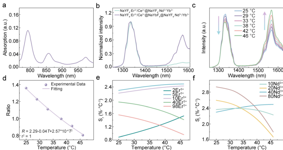
Fig. 2 (a) Absorption spectra of the NPs. (b) Normalized emission spectra of NaYF 4 :5Er 3+ /2Ce 3+ @NaYF 4 :40Nd 3+ /20Yb 3+ and NaYF 4 :5Er 3+ /2Ce 3+ @NaYbF 4 @NaYF 4 :40Nd 3+ /20Yb 3+ . (c) Temperature dependence of the emission spectra of NaYF 4 :5Er 3+ /2Ce 3+ @NaYbF 4 @NaYF 4 :40Nd 3+ /20Yb 3+ . (d) Temperature dependence of the intensity ratio between the emission at 1330 and 1565 nm. The acquired S_r values of (e) NaYF 4 , x Er 3+ /2Ce 3+ @NaYbF 4 @NaYF 4 ,40Nd 3+ /20Yb 3+ nanoparticles with varied Er 3+ concentrations and (f) NaYF 4 ,5Er 3+ /2Ce 3+ @NaYbF 4 @NaYF 4 , y Nd 3+ /20Yb 3+ nanoparticles with varied Nd 3+ concentrations. All temperature-dependent spectra were measured in an aqueous environment.
