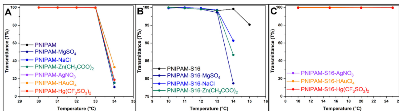
Fig. 5 Transmittance of aqueous solutions of (A) PNIPAM (1.0 mg mL -1 , λ = 700 nm) containing NaCl, Zn(CH 3 COO) 2 , MgSO 4 , Hg(CF 3 SO 3 ) 2 , AgNO 3 and HAuCl 4 . Transmittance of aqueous solutions of PNIPAM-S16 (1.0 mg mL -1 , λ = 700 nm) containing (B) NaCl, Zn(CH 3 COO) 2 and MgSO 4 and (C) Hg(CF 3 SO 3 ) 2 , AgNO 3 and HAuCl 4 .
