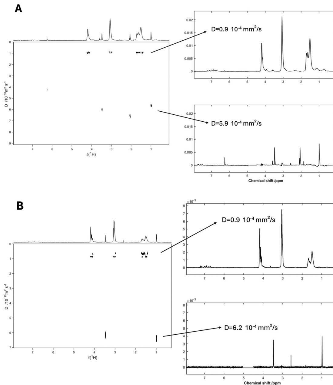
Fig. 4 (A) DOSY ^1\text{H} spectrum (left) of Arg 9 -P54 suspension in deuterated water at 25 °C after filtration through a 0.2 μm filter and the corresponding two-component SCORE analysis (right) and (B) DOSY ^1\text{H} spectrum (left) of Arg 9 -P819 suspension in deuterated water at 25 °C after filtration through a 0.2 μm filter and the corresponding two-component SCORE analysis (right).
