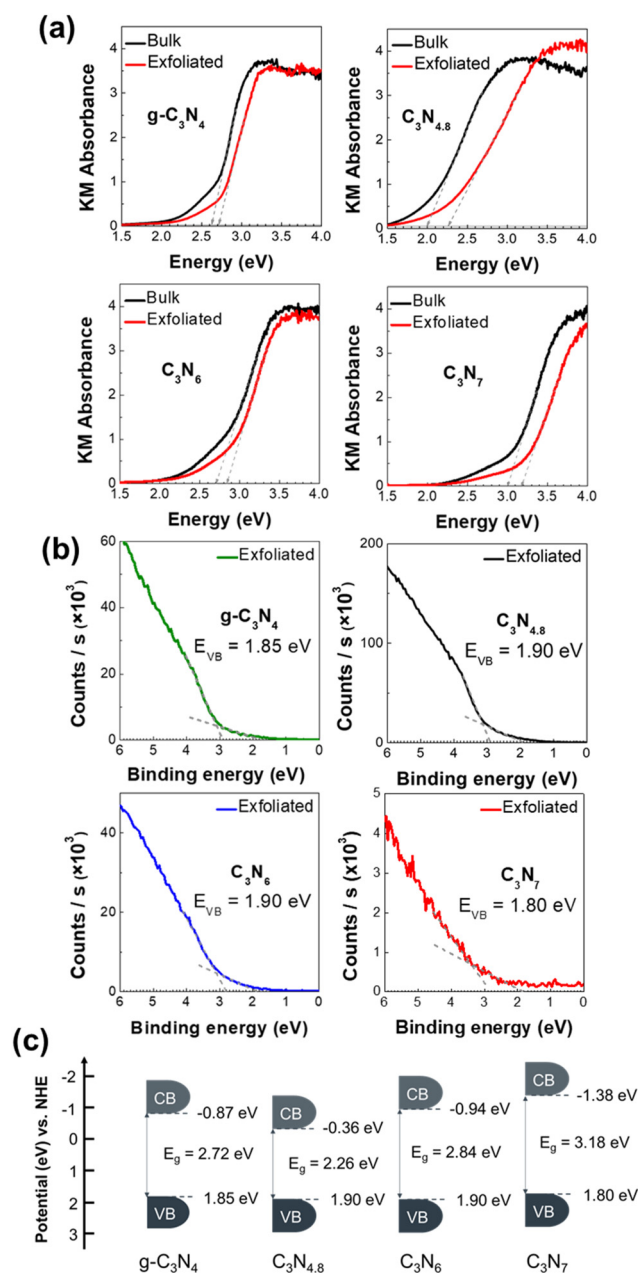
Fig. 5 (a) UV-Vis absorption spectra, (b) UPS spectra, and (c) schematic illustration of the band position for exfoliated g-C_3N_4 , C_3N_{4.8} , C_3N_6 , and C_3N_7 nanosheets.
