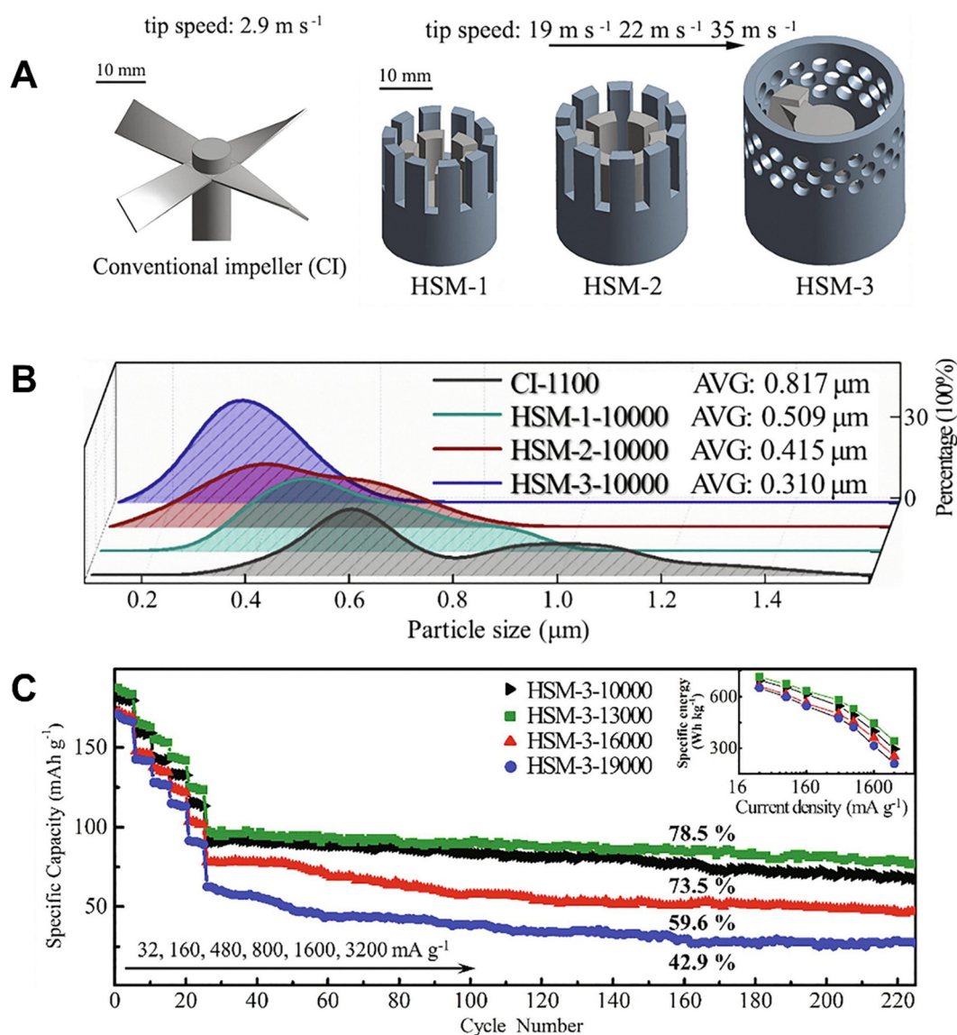
Fig. 14 (A) Conventional impeller (left), three HSM mixing heads with rotor–stator teathed (HSM-1, HSM-2), and blade-screen configuration (HSM-3) (right). (B) Particle size distribution of the synthesized samples. (C) Rate capabilities, specific discharge energies (inset) and cycling stabilities at various current densities. Adapted with permission from ref. 67. Copyright 2021 Elsevier. 67
