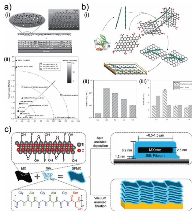
Fig. 6 (a) (i) Schematic illustration of self-assembly for nacre-like composites of silk fibroin and GO crystals. (ii) Mechanical properties of nacre-like composites of nacre-like composites of silk fibroin and GO crystals. Adapted with permission. 134 Copyright 2013, Wiley-VCH. (b) (i) Schematic illustration of self-assembly for nacre-like composites of amyloid fibrils and GO crystals. (ii) Conductivity of nacre-like composites of amyloid fibrils and GO crystals. (iii) Tensile modulus of nacre-like composites of amyloid fibrils and GO crystals. Adapted with permission. 45 Copyright 2015, Springer Nature. (c) Schematic illustration of self-assembly for nacre-like composites of silk and MXene crystals. Adapted with permission. 51 Copyright 2020, Wiley-VCH.
