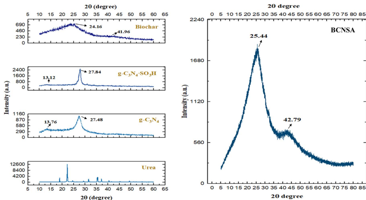
Fig. 3 The XRD graph of urea, g\text{-C}_3\text{N}_4 , g\text{-C}_3\text{N}_4\cdot\text{SO}_3\text{H} , biochar and the synthesized BCNSA catalyst.
