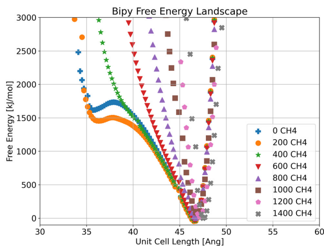
Fig. 3 Visualization of crystalline ZnMOP-bipy system and free energy landscape of the system as a function of unit cell side length and methane loading in molecules per unit cell.
