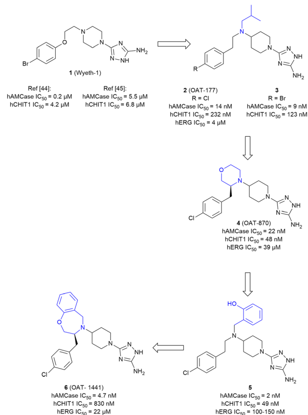
Fig. 4 Evolution of aminotriazole-based AMCase inhibitors.
