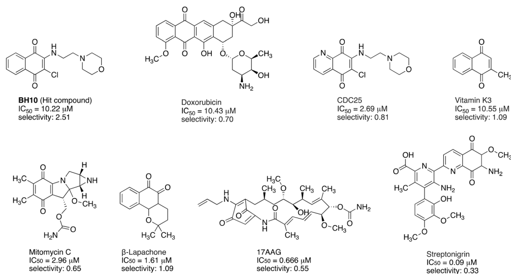
Fig. 2 Chemical structure and biactivity of BH10 and seven other well-known anticancer compounds. IC 50 values ( \mu M) indicate the cytotoxicity towards HEC1A endometrial cancer cells, while selectivity is calculated as the IC 50 value for non-cancerous MAD11 cells divided by the IC 50 value for HEC1A cells. 7
