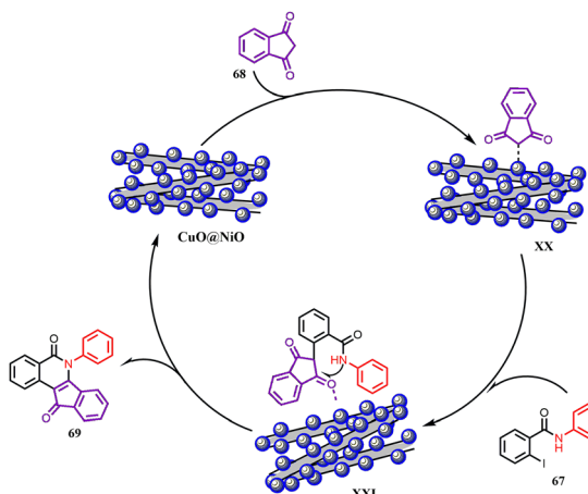
Fig. 8 Plausible mechanism for synthesis of indenoisoquinolines using a CuO@NiO nanocatalyst.
