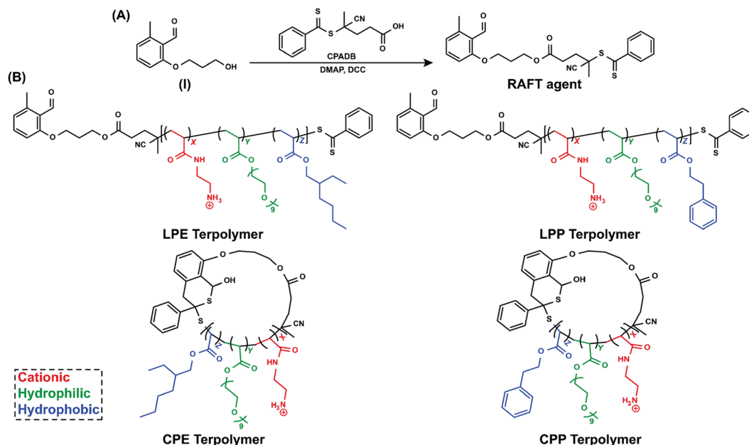
Fig. 16 (A) Synthesis scheme of RAFT agent. (B) Chemical structures of amphiphilic LPE , CPE , LPP , and CPP ( X = percentage of cationic groups, Y = percentage of hydrophilic groups, and Z = percentage of hydrophobic groups). Redrawn from ref. 158.
