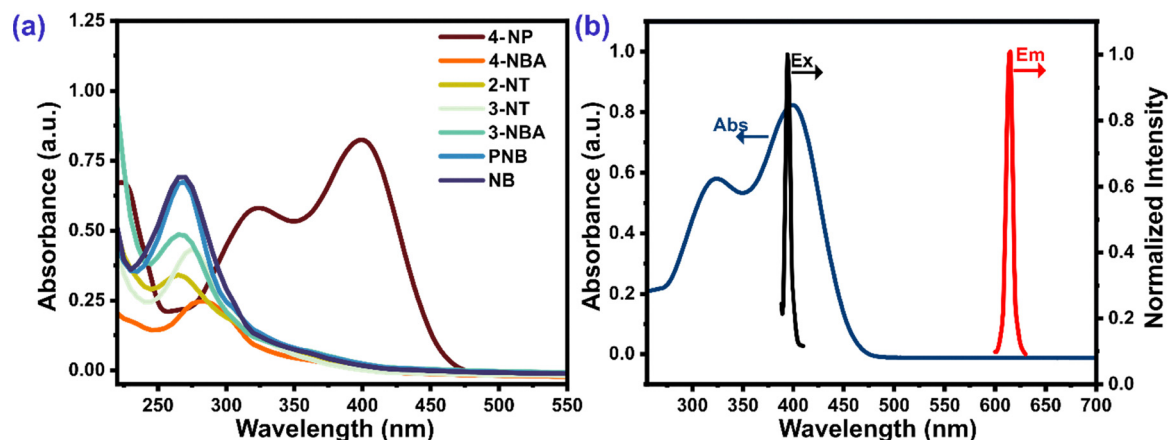
Fig. 9 (a) UV-vis absorption spectra of different nitroaromatic compounds. (b) UV-vis absorption spectra of 4-NP and excitation and emission spectra of the ZELMO phosphor dispersed in deionized water.
