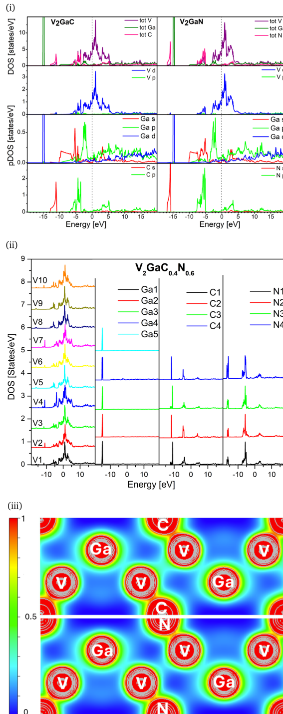
Fig. 3 (i) Calculated density of states for V_2GaC (on the left) and V_2GaN (on the right). The top panel shows the total density of states, followed by the partial DOS of V, Ga, and C/N, which are color-coded. (ii) Represents calculated total DOS for nonequivalent atom sites present in (carbo)nitride phase V_2GaC_{0.4}N_{0.6} . (iii) Calculated valence electron density of V_2GaC (top) and V_2GaN (bottom) in the (110) plane. This plane was selected to visualize the V, Ga, and C/N bonding scheme. The map is depicted by an isosurface of 0.827 with a minimum and maximum cutoff value of 0.018 and 0.998, respectively.
