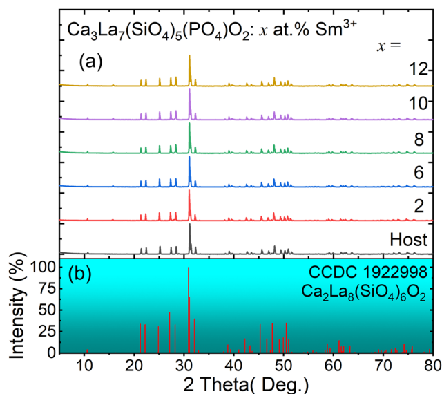
Fig. 1 (a) XRD patterns of \text{Ca}_3\text{La}_7(\text{SiO}_4)_5(\text{PO}_4)\text{O}_2 with different doping concentrations of Sm 3+ ions (0–12 at%); (b) standard powder diffraction card of \text{Ca}_2\text{La}_8(\text{SiO}_4)_6\text{O}_2 ; reference plot was downloaded from CCDC database, file number 1922998 (ICSD 140674).
