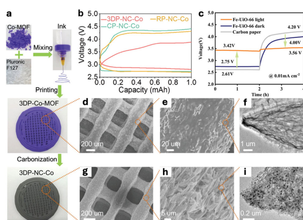
Fig. 21 (a) Diagram showing the preparation of a 3DP Co-MOF-derived framework. (b) Comparison of the charge overpotential with the marked cathodes at a limited capacity of 1 mAh and current density of 0.1 mA cm -2 . (c) Discharge and charge profiles of the Li-O 2 battery with and without illumination. (d-f) Typical characterization of 3DP-Co-MOF. (d and e) SEM images. (f) TEM image. (g-i) Typical characterization of 3DP-NC-Co. (g and h) SEM images. (i) TEM image. (a and b) and (d-i) reproduced with permission. 135 © 2018, WILEY-VCH Verlag GmbH & Co. KGaA, Weinheim. (c) Reproduced with permission. 136 © 2024, Wiley-VCH GmbH.
