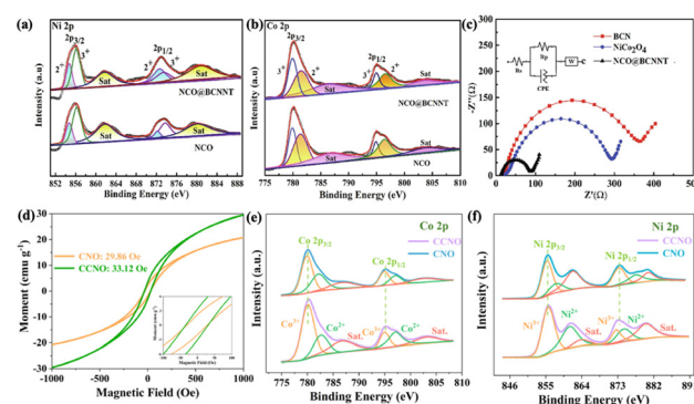
Fig. 8 High-resolution XPS spectra of (a) Ni 2p and (b) Co 2p. (c) Nyquist plots of batteries in the frequency range of 10^{-5} – 10^{-2} Hz. Reproduced with permission. 196 Copyright 2021, Elsevier. (d) Magnetic field dependence of magnetization ( M-H ) profiles of CNO and CCNO at 300 K (the inset shows a partial enlarged image). (e) Co 2p and (f) Ni 2p spectra of CNO and CCNO. Reproduced with permission. 198 Copyright 2022, Elsevier.
