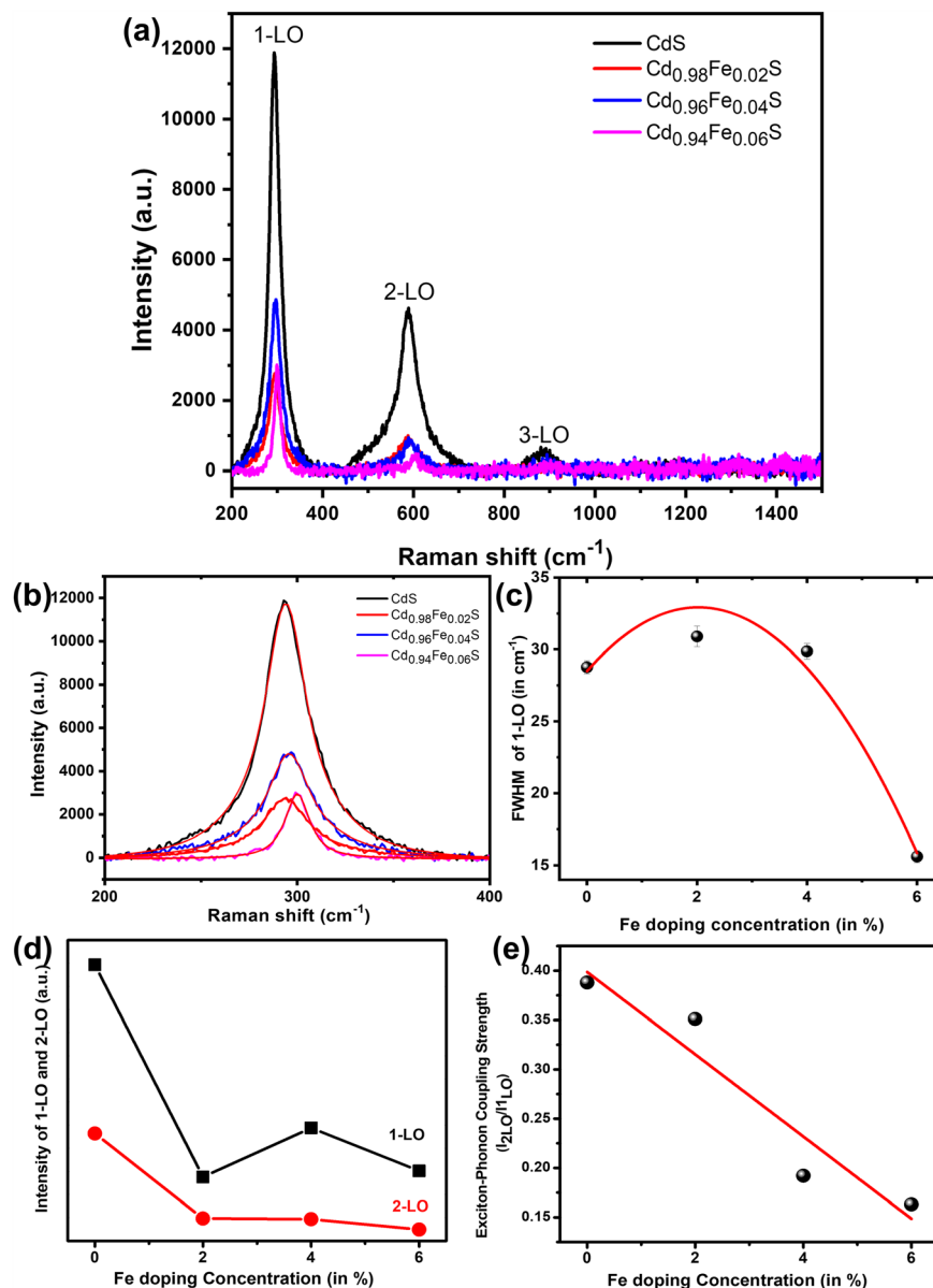
Fig. 6 (a) Raman spectra of Cd 1-x Fe x S quantum dots at room temperature, (b) Raman spectra of Cd 1-x Fe x S quantum dots: 1-LO (fitted to get the exact peak position), (c) FWHM variation (1-LO) with Fe doping concentrations, (d) relative Raman intensity of 1-LO with increasing Fe doping concentrations, (e) variation in exciton-phonon coupling strength with Fe doping concentration.
