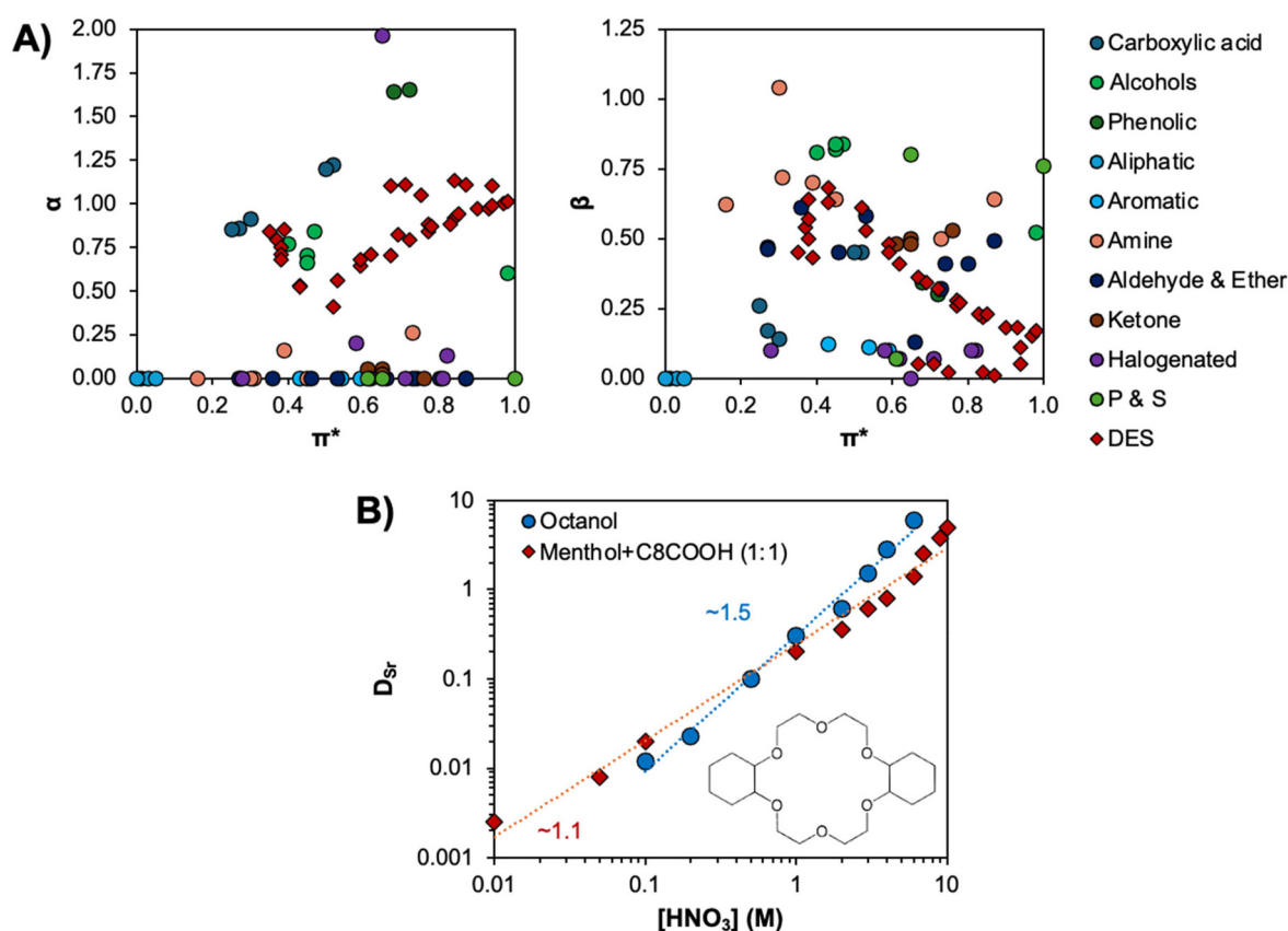
Fig. 11 (A) Plot of binary experimental Kamlet–Taft parameters of organic solvents and non-ionic eutectic solvents. Organic solvent parameters were obtained from the Marcus database, 154 whilst those of DESs are available in Table S5.† (B) Comparison of the effect of nitric acid on the solvent extraction of Sr^{2+} by 0.1 mol L −1 dicyclohexano-18-crown-6 ether in either octanol or a mixture of nonanoic acid and menthol. This figure has been adapted from ref. 147 with permission from Elsevier, copyright 2022.
