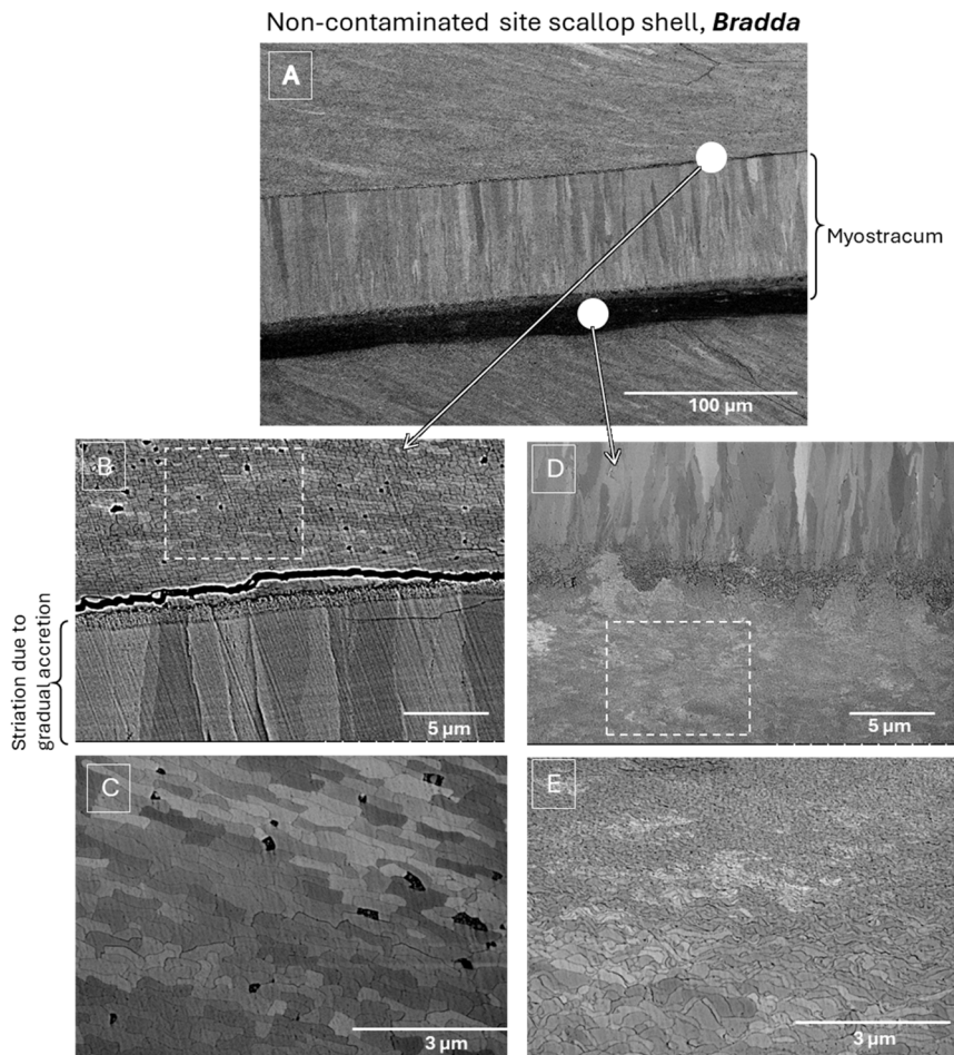
Fig. 4 BSE micrographs of the myostracum region for the scallop shell collected in the non-contaminated Bradda area. (A) A general view of the region of interest. (B) The upper boundaries between the myostracum and the shell bulk. (C) The microstructures of the scallop in the region at the top of the myostracum. (D) The lower boundaries between the myostracum and the shell bulk. (E) The microstructures of the shell in the region below the myostracum.
