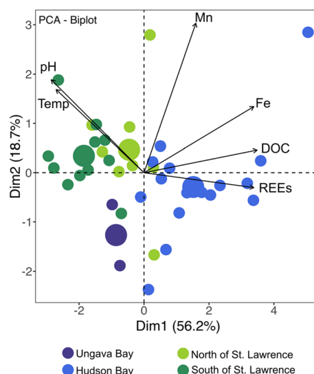
Fig. 3 Principal component analysis in type 2 framing with filtered concentrations of elements in rivers draining the different watersheds of the Province of Québec. Larger circles represent the center of each group distribution.
