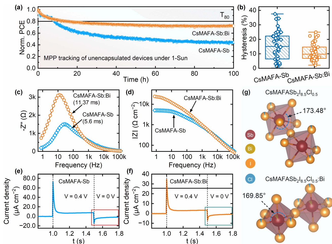
Fig. 6 Aging studies of unencapsulated CsMAFA-Sb and CsMAFA-Sb:Bi solar cells in a N_2 atmosphere. (a) MPP tracking of both devices under 1-Sun illumination at room temperature (RT \approx 28 °C). The initial PCEs of the CsMAFA-Sb and CsMAFA-Sb:Bi devices are 2.5% and 2.2%, respectively. (b) Distribution of hysteresis index of both the devices. Hysteresis index = (PCE_{REV}/PCE_{FOR}) \times 100\% - 100\% . (c) Imaginary impedance as a function of frequency. (d) Magnitude of impedance as a function of frequency for both devices. (e) Transient dark current curves of (e) CsMAFA-Sb and (f) CsMAFA-Sb:Bi devices. Two regions of voltage application of 0.4 V and 0 V are shown. The ionic charge was estimated using: Q_{ion} = \int_{V=0} V dt . (g) The I-Sb(Bi)-I angles in the pnictogen halide octahedra from the crystal structures of CsMAFA-Sb and CsMAFA-Sb:Bi, which were determined using Rietveld refinement of the corresponding XRD patterns.
