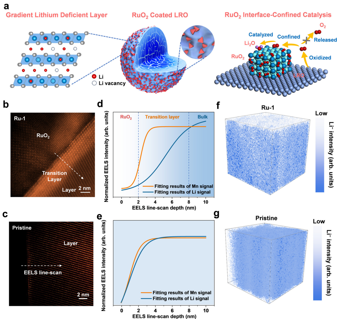
Fig. 1 (a) Schematic diagram of the gradient lithium-deficient layer and RuO 2 interface-confined catalysis in Ru-1. Characterization of a lithium-deficient layer. HADDF-STEM images of (b) Ru-1 and (c) the pristine sample. The normalized EELS intensities of the line-scan from the surface to the bulk of (d) Ru-1 and (e) pristine samples. The 3D plots of the TOF-SIMS Li + intensity of (f) Ru-1 and (g) pristine samples. The blue region corresponds to the high Li content.
