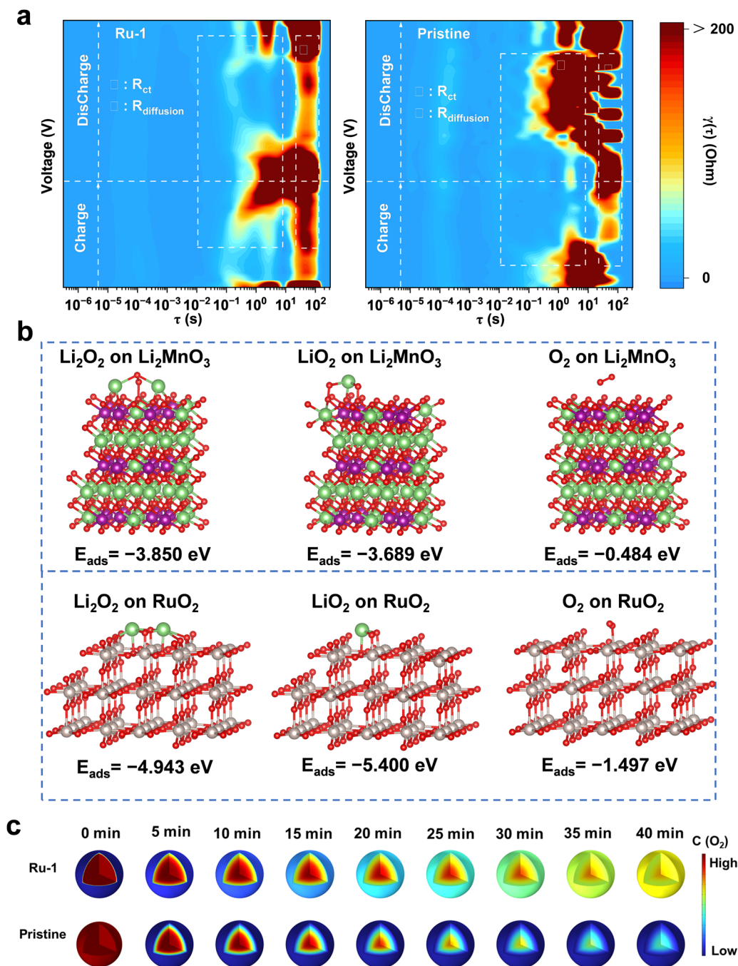
Fig. 6 The adsorption and catalytic capability evaluation. (a) DRT profile transformation from GEIS of Ru-1 and the pristine sample. (b) The models and adsorption energies of \text{Li}_2\text{O}_2 , \text{LiO}_2 , and \text{O}_2 adsorbed on \text{Li}_2\text{MnO}_3 and \text{RuO}_2 . (c) \text{O}_2 diffusion simulation of Ru-1 and the pristine sample with COMSOL software.
