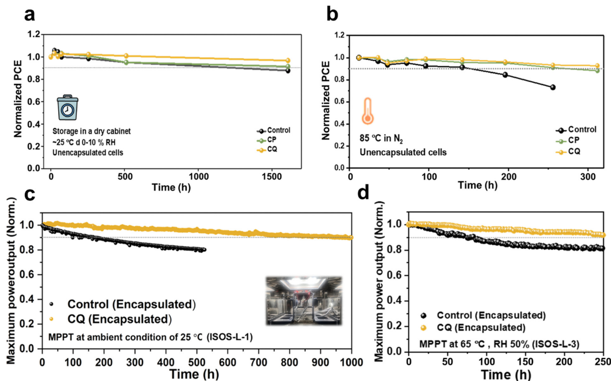
Fig. 7 Stability evaluation. (a) Storage stability of the control, CP-, and CQ-treated PSCs stored in a dry cabinet ( \sim 25 °C, RH of \sim 10\% ). (b) Thermal stability test of the control, CP-, and CQ-treated PSCs ( \sim 85 °C, N 2 -filled glovebox). MPPT testing for the control and CQ-treated PSCs using (c) ISOS-L-1 and (d) ISOS-L-3, which was measured under full solar illumination (AM 1.5 G, 100 \text{ mW cm}^{-2} ) without a UV filter.
