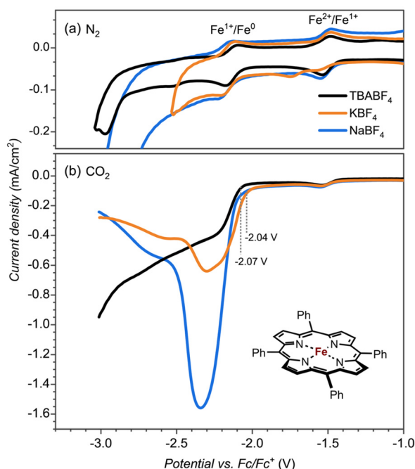
Fig. 2 Cyclic voltammetry (CV) of [\text{Fe}^{\text{III}}(\text{TPP})]^+ ( 0.25 mM) measured in electrolytes containing \text{TBABF}_4 (black), \text{NaBF}_4 (blue) and \text{KBF}_4 (orange) ( 0.1 M in \text{DMF} + 0.5\text{M} \text{H}_2\text{O} ; scan rate 100 mV \text{s}^{-1} ) under (a) \text{N}_2 and (b) \text{CO}_2 .
