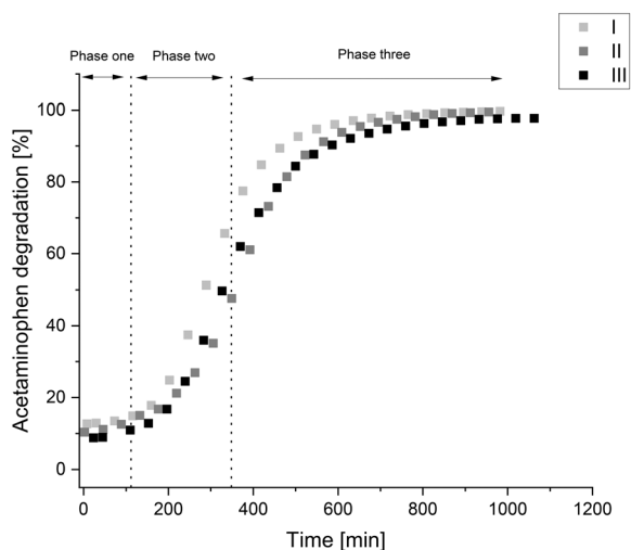
Fig. 6 Change in detected acetaminophen degradation over time for three samples which were treated by the electro-Fenton process and continuously kept at 25^\circ\text{C} for measurement by HPLC.
