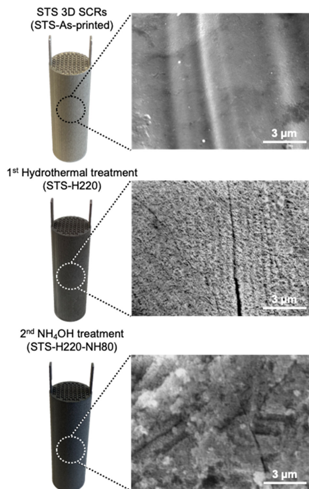
Fig. 2 Photographs and SEM images of STS 3D SCRs before and after each treatment step. The scan speed for the 3D printing process is 1200\text{ mm s}^{-1} .
