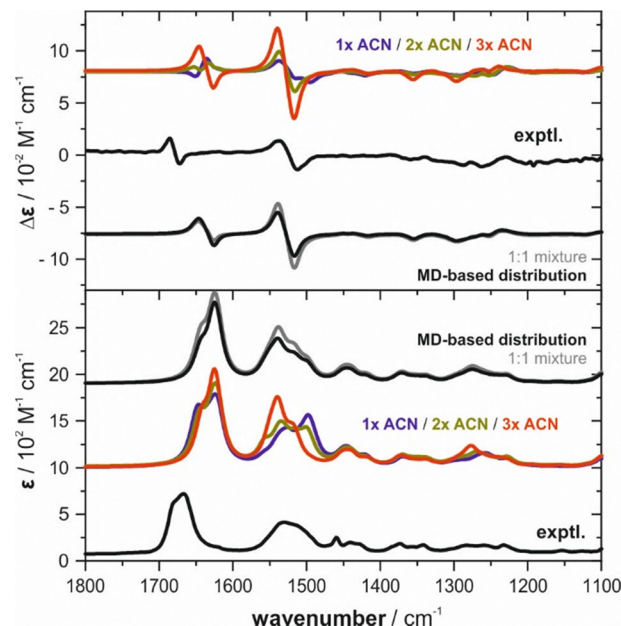
Fig. 5 Comparison of the experimental and computed VCD and IR spectra of (S)- Ace-Trp-N(n-Pr) in ACN- d_3 (0.077 M, 200 \mu m) with computed spectra of the single, double and triple solvated structures, a 1 : 1 mixture of double and triple solvated state, and an MD-based conformational distribution.
