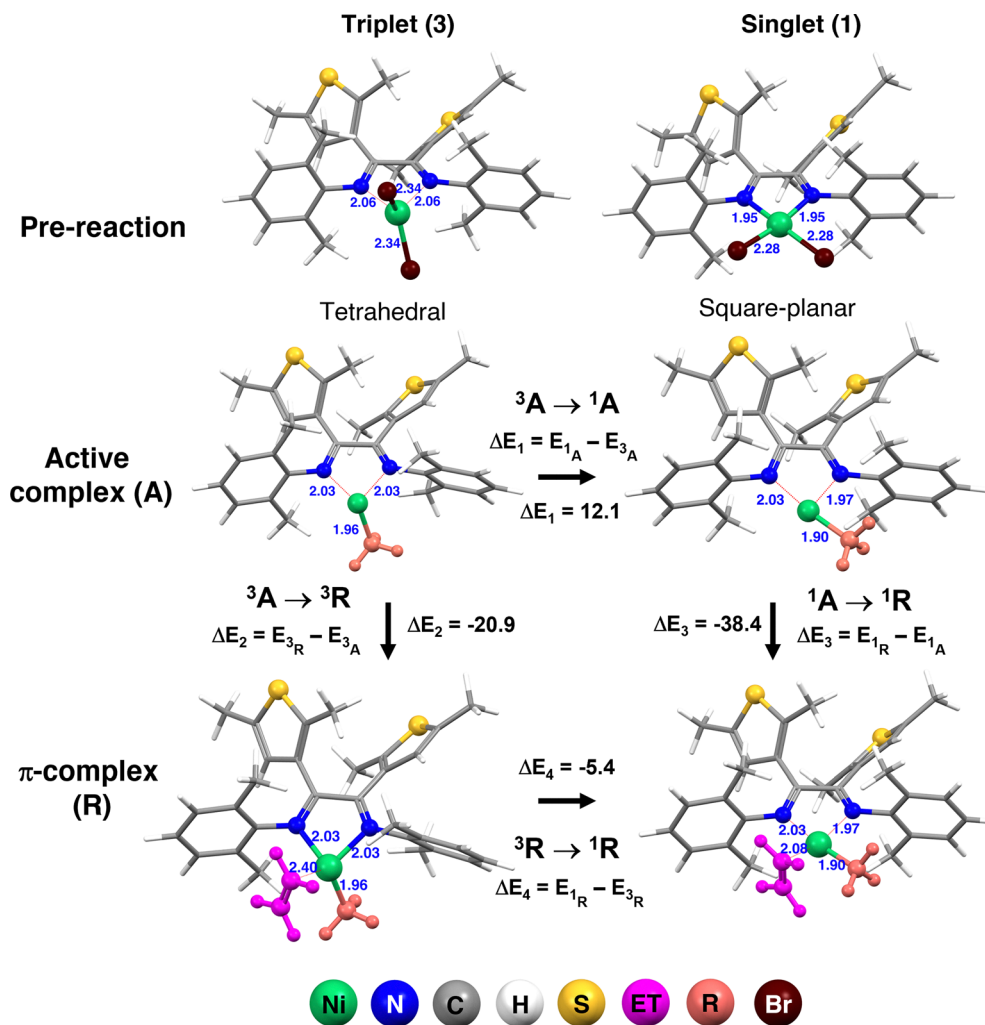
Fig. 4 The pre-catalyst complex, active complex, and \pi -complex in the singlet and the triplet states. The energy for each state is given in \text{kcal mol}^{-1} .
