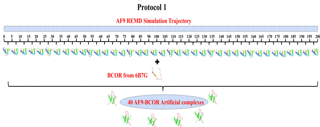
Fig. 2 Schematic representation of Protocol 1 for the preparation of AF9–BCOR artificial complexes.
