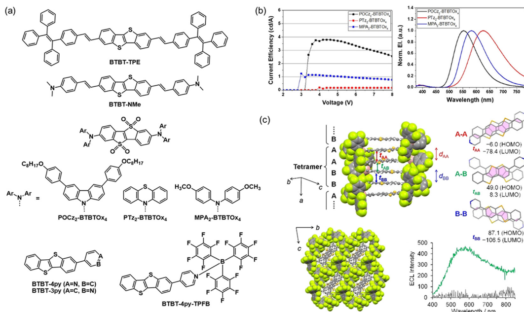
Fig. 12 (a) Structures of BTBT-based luminescent molecules. (b) The current efficiency and electroluminescence spectra of OLEDs using POCz 2 -BTBTOn, PTz 2 -BTBTOn and MPA 2 -BTBTOn as emitting layers. Reprinted with permission from ref. 104. Copyright 2025, The Royal Society of Chemistry. (c) Crystal structures of BTBT-4py-TPFB with transfer integral values and electrochemiluminescence from the crystalline film of BTBT-4py-TPFB with a co-reactant in PBS aqueous solutions. Reprinted with permission from ref. 97. Copyright 2023, Wiley-VCH.
