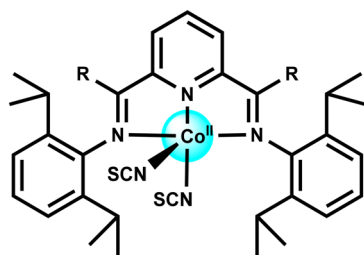
Fig. 4 Schematic representation of complexes 1a and 1b . 67
