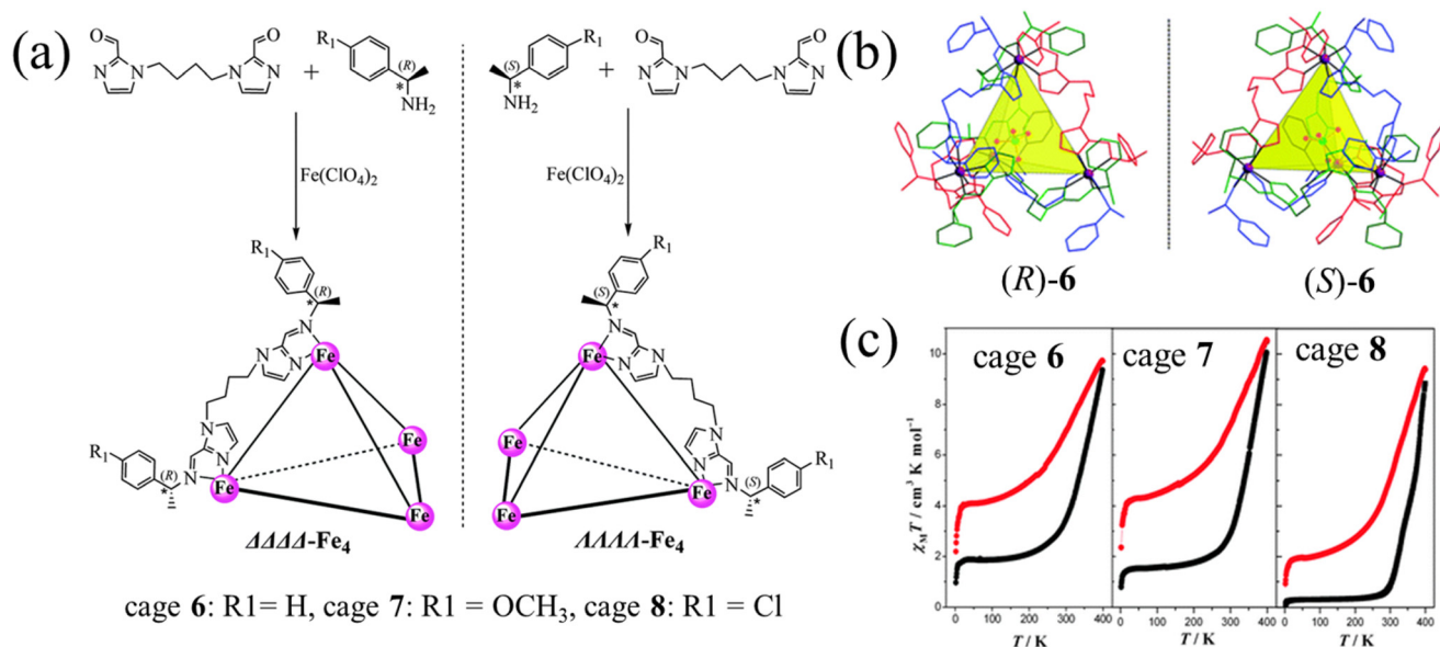
Fig. 8 (a) Synthesis method of 6–8. (b) Crystal structures of 6. (c) \chi_m T vs. T plots for 6–8. 79
