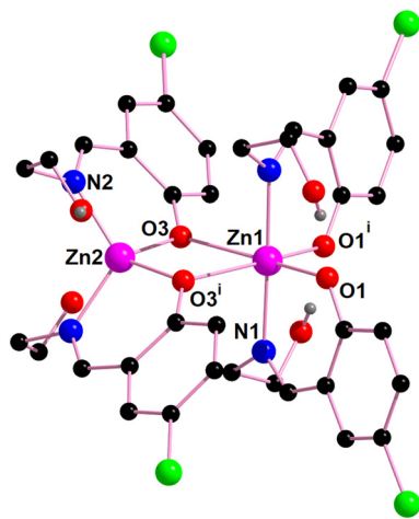
Fig. 8 Perspective view of complex 3 with selective atom numbering. Symmetry transformation \text{i} = 1 - x, y, 1.5 - z .
