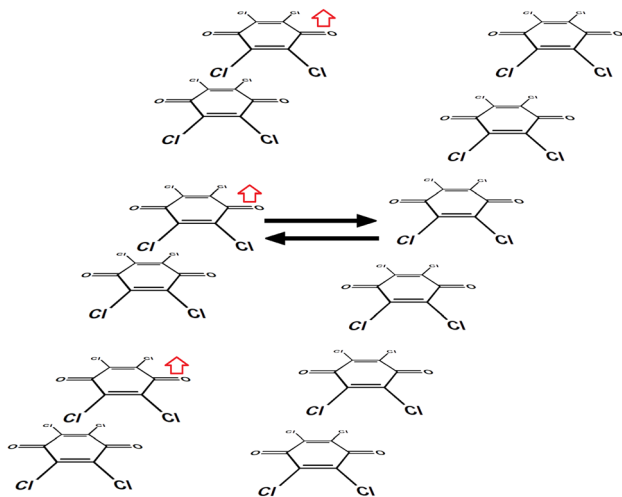
Fig. 5 A stack of pancake-bonded dimers (left) of tetrachlorosemiquinone radical anions transforms into a stack of equidistant tetrachlorosemiquinone radical anions (right). 68 A spin-Peierls transformation requires adjustment of positions of one radical anion in each dimer (marked by a red arrow).
