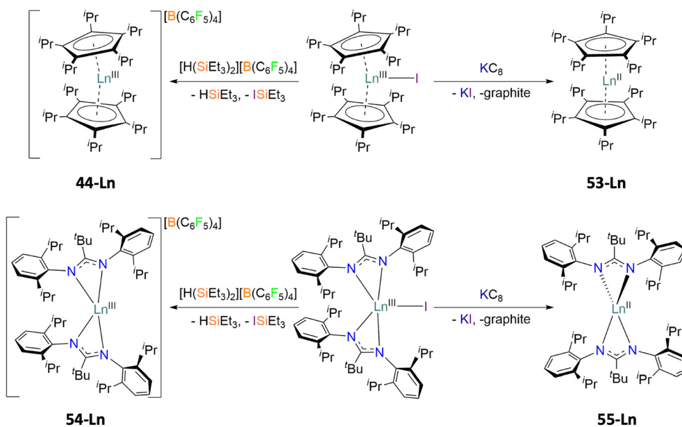
Fig. 8 Synthetic routes and structural differences of the cationic lanthanocenium ion [Ln(Cp iPr5 ) 2 ][B(C 6 F 5 ) 4 ] 44-Ln versus the neutral lanthano-cene molecule [Ln(Cp iPr5 ) 2 ] 53-Ln (top), and the bis-amidinate complexes [Ln(Piso) 2 ][B(C 6 F 5 ) 4 ] 54-Ln and [Ln(Piso) 2 ] 55-Ln (bottom), Ln = Dy, Tb. 75,76
