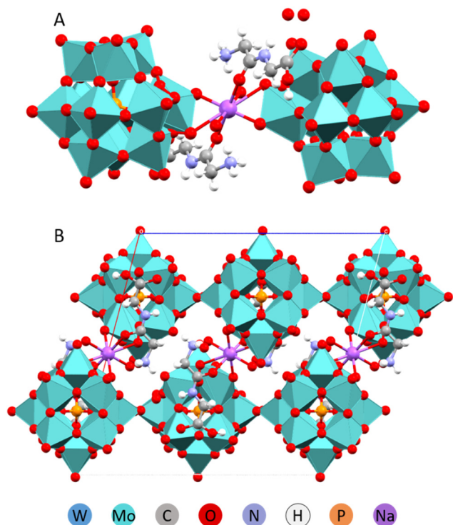
Fig. 5 Molecular (A) and crystal (B) structures of the Na(HGlyGly)(H 3 O)[PMo 12 O 40 ] \cdot 3H 2 O compound. 31
