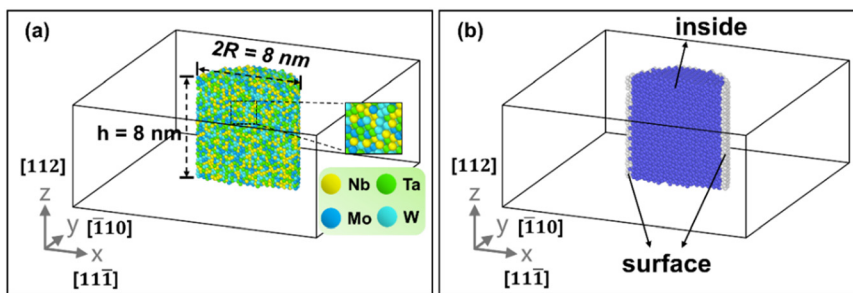
Fig. 1 Atomic configuration and cross-section of the NbMoTaW RHEA nanowire with a radius ( R ) of 4 nm and the loading direction of [112]. (a) Cross-section with atoms colored by the element type. (b) Cross-section with atoms colored by the local structure, with blue and white balls denoting inner and surface layer atoms, respectively.
