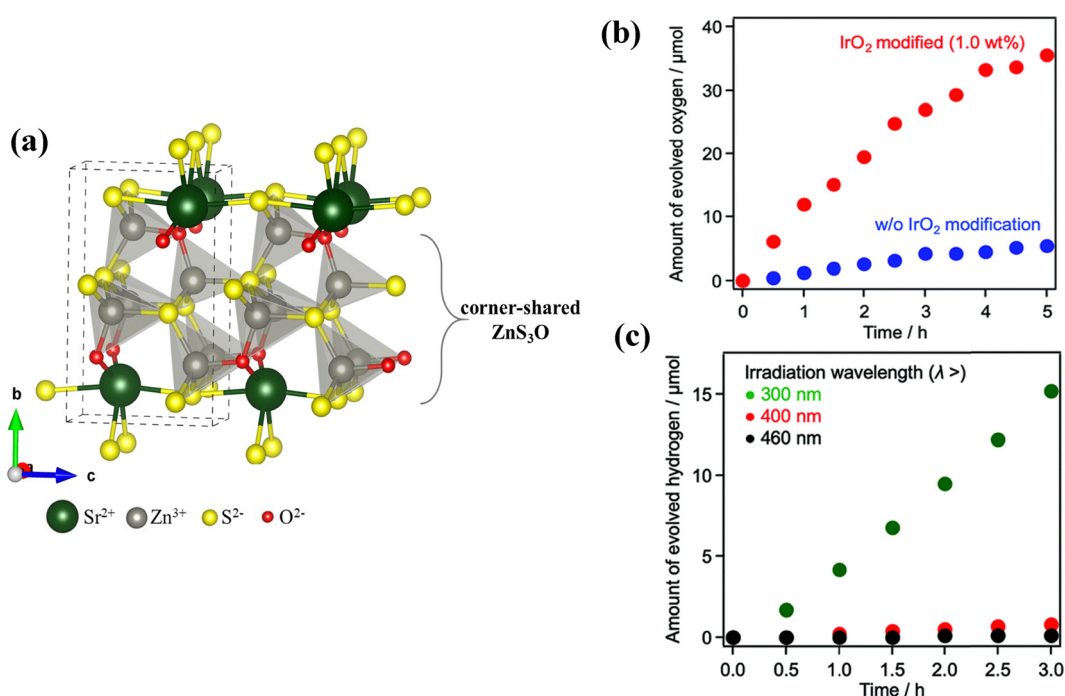
Fig. 4 (a) Structural representation of SrZn 2 S 2 O oxysulfide of Pmn 2 1 symmetry; (b) oxygen evolution for SrZn 2 S 2 O and (c) hydrogen evolution for Pt/SrZn 2 S 2 O. Reproduced from ref. 92 with permission from the Royal Society of Chemistry.
