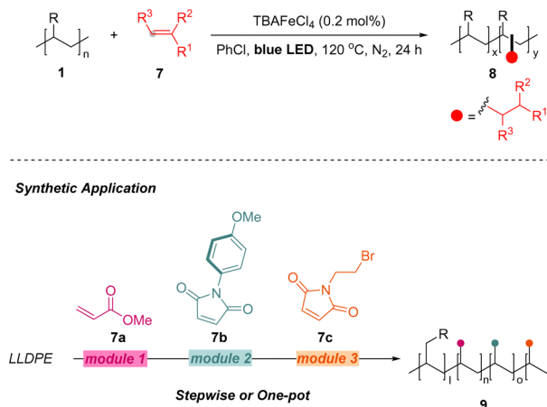
Scheme 5 Photoinduced iron-catalysed C–H alkylation of polyolefins.
