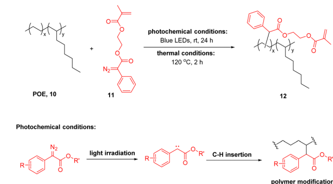
Scheme 6 Carbene-mediated C–H functionalization of polymers.
