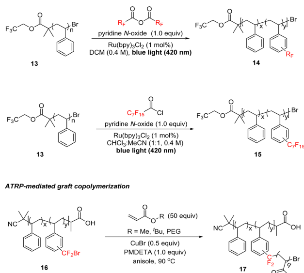
Scheme 7 Photocatalysed C–H fluoroalkylation of aromatic polymers.
