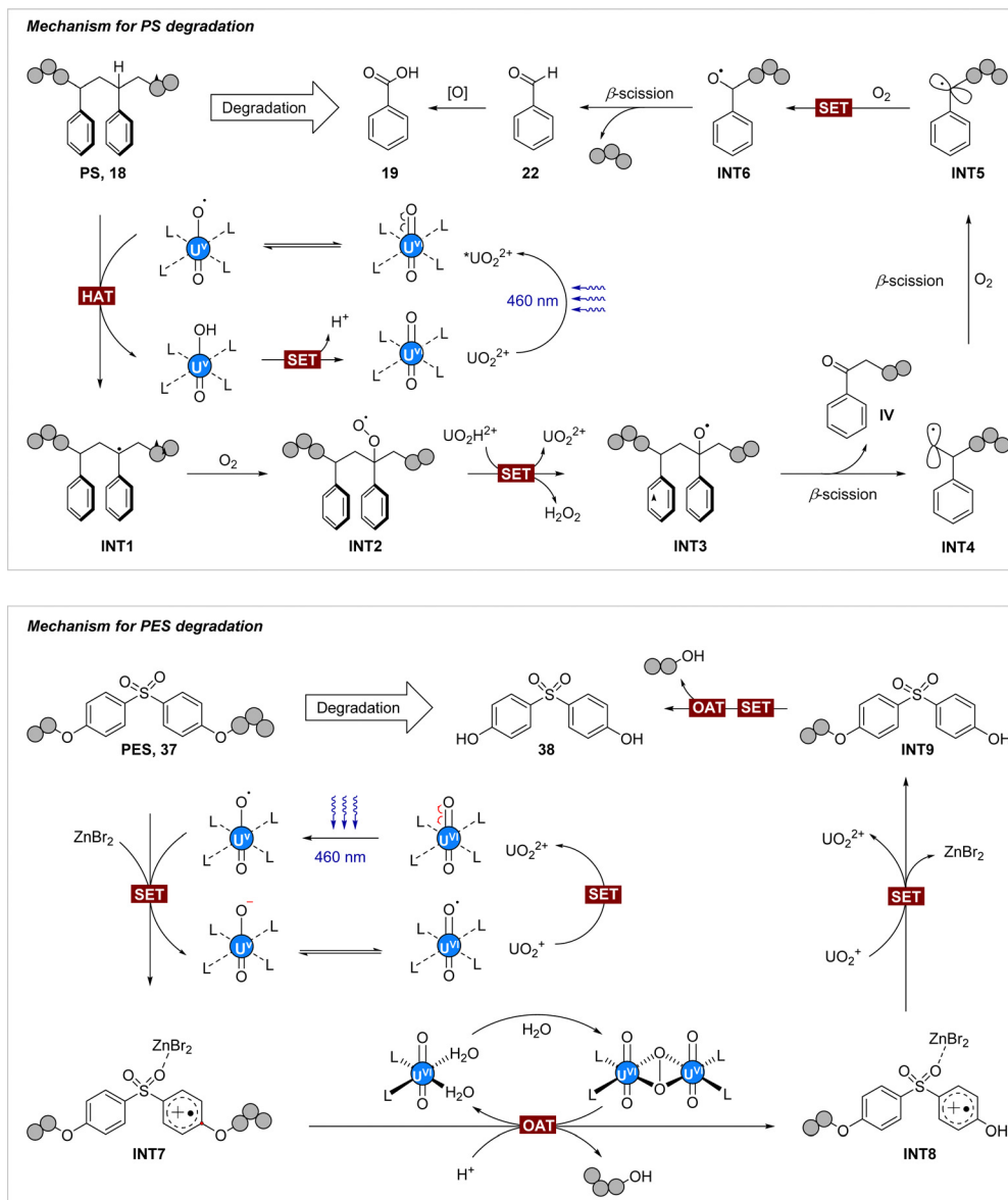
Scheme 13 Possible mechanism for degradation of plastic wastes with uranyl-photocatalyst under visible light.
