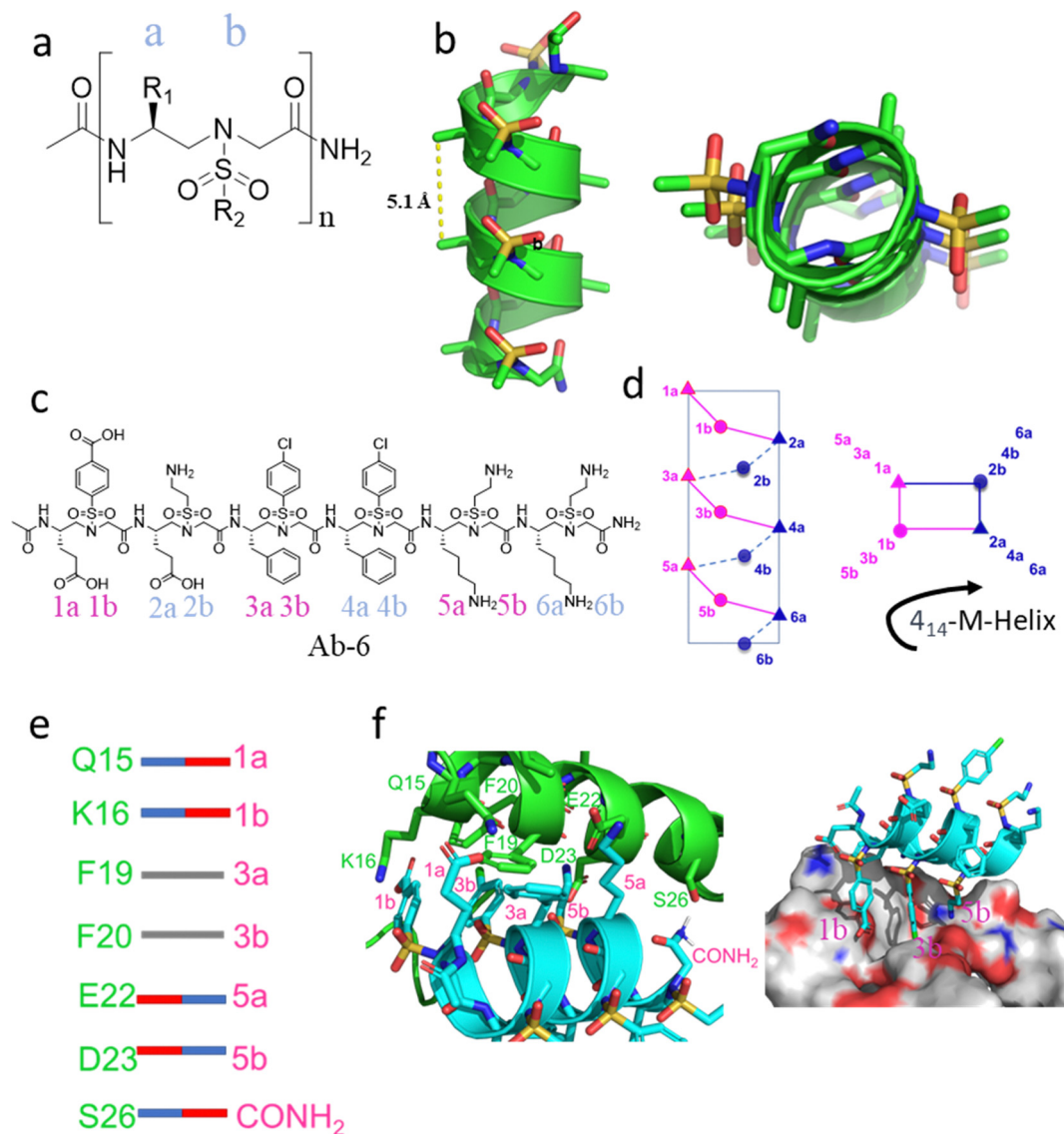
Fig. 5 (a) Chemical structures of sulfonyle- \gamma -AApeptides: "a" and "b" denote the chiral and sulfonyle side chains. (b) Side and top views of sulfonyle- \gamma -AApeptides. (c) Chemical structure of Ab-6 . (d) Helical wheel of sulfonyle- \gamma -AApeptide illustrating side chain distribution. (e) and (f) Hypothesized interactions between Ab-6 and A \beta side chains.
