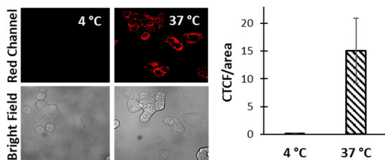
Fig. 2 Impact of metabolic activity on GluRho uptake. Fluorescence and bright field images present probe-treated (2 \mu M) MCF7 cells pre-conditioned at 37 ^{\circ} C vs. 4 ^{\circ} C for 15 min. Images were acquired using a confocal microscope, 60 \times objective, and recorded at exc. 559 nm/em. 603 nm under identical imaging parameters. Graph presents fluorescence quantified from the respective images using ImageJ as CTCF/Area: CTCF = (Integrated Density – (Area of selected cell \times Mean fluorescence of background readings))/Area of the selected cell. Error bars represent the standard deviation.
