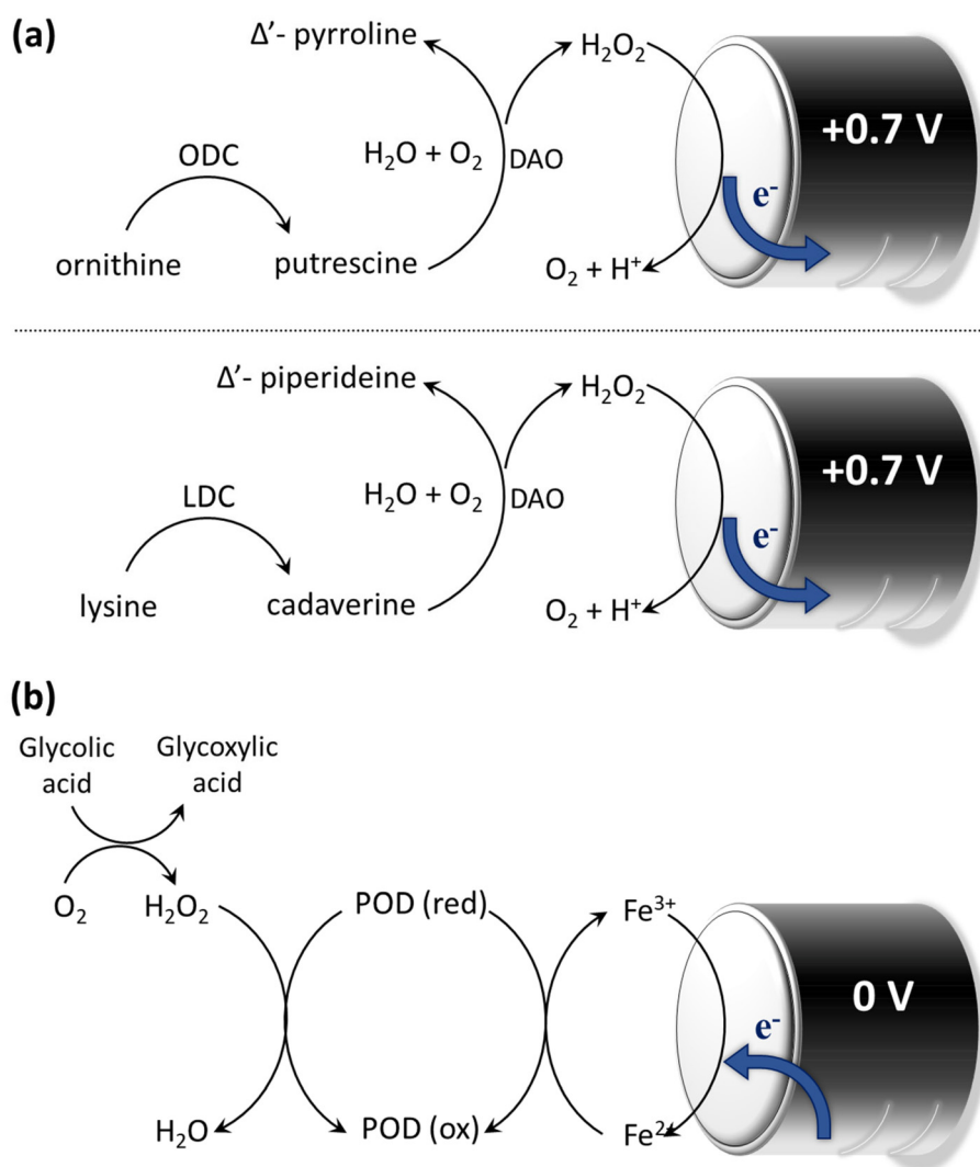
Fig. 37 Enzymatic mechanisms in (a) the legume cotyledon tissue biosensors (reproduced from ref. 285 with permission from Elsevier, Copyright 1993) and (b) ferrocene-mediated spinach tissue-based biosensor. (Reproduced from ref. 293 with permission from Elsevier, Copyright 1994.)
