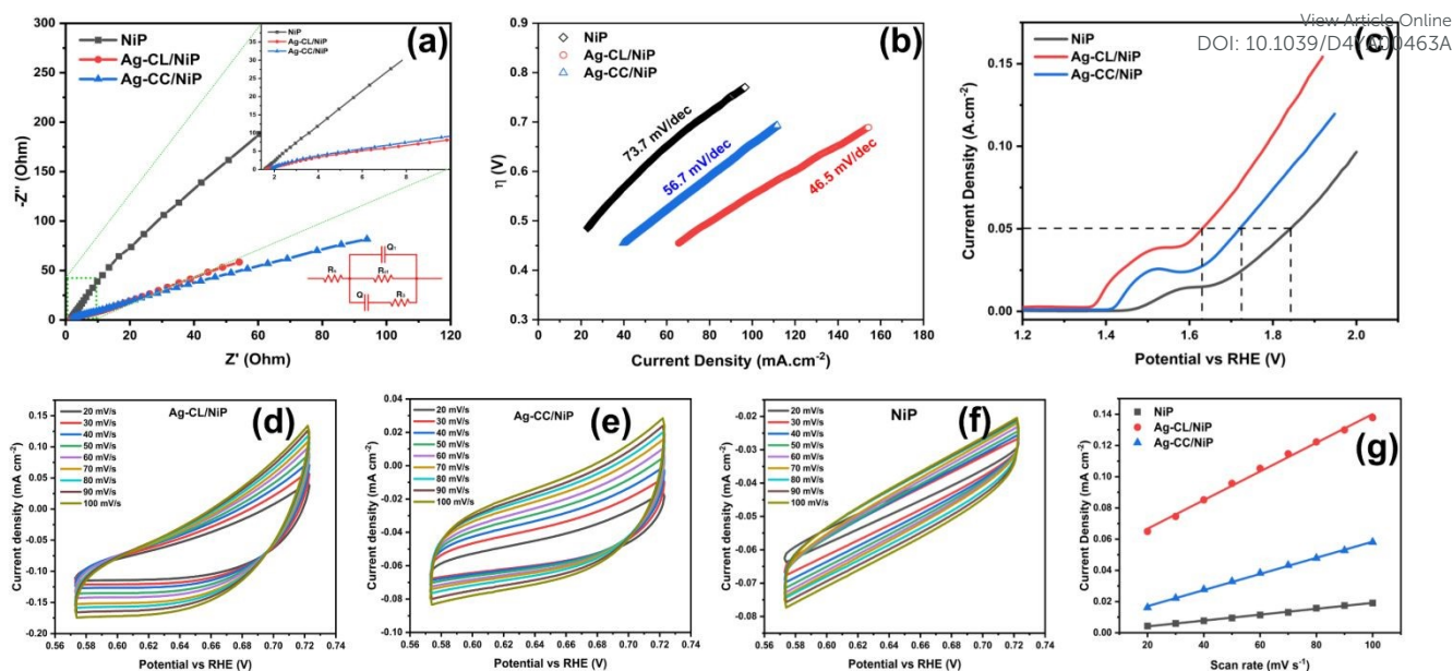
Figure 5: (a) Nyquist plot and equivalent circuit (b) Tafel curves (c) LSV curves. Analysis of the electrochemically active surface area (ECSA): CV curves of (d) Ag-CL/NiP (e) Ag-CC/NiP (f) NiP. Determination of C_{dl} using (g) the plot of double layer charging current density variation vs. scan rate by a linear regression of Ag-CL/NiP, Ag-CC/NiP and NiP.
