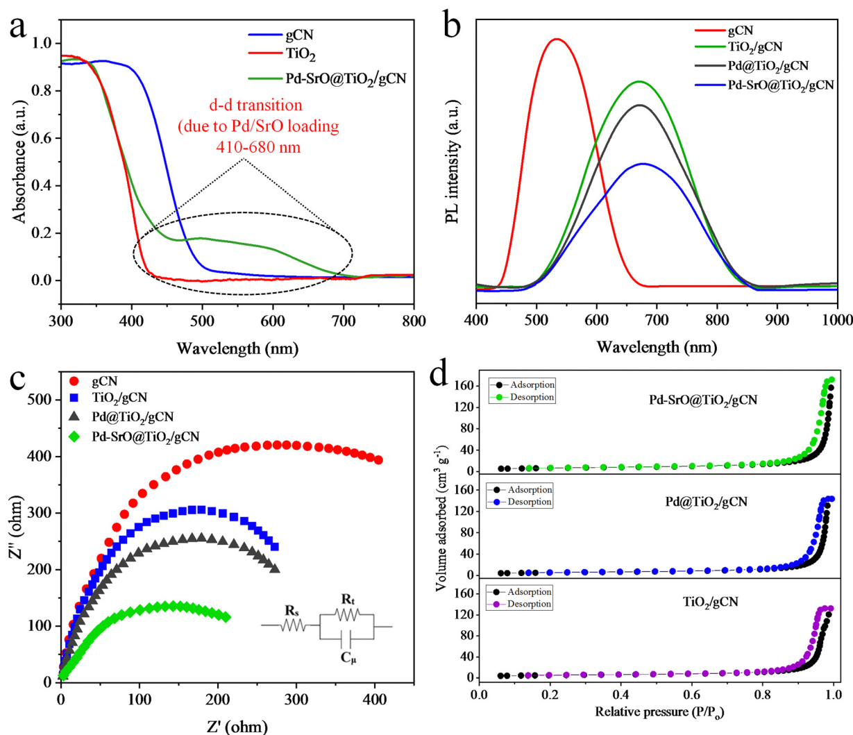
Fig. 2 (a) UV-DRS spectra of \text{TiO}_2 , gCN and \text{Pd-SrO@TiO}_2/\text{gCN} ; (b) PL spectra at the excitation wavelength of 325 nm; (c) EIS results of gCN, \text{TiO}_2/\text{gCN} , \text{Pd@TiO}_2/\text{gCN} , and \text{Pd-SrO@TiO}_2/\text{gCN} ; (d) BET analyses of \text{TiO}_2/\text{gCN} , \text{Pd@TiO}_2/\text{gCN} and \text{Pd-SrO@TiO}_2/\text{gCN} .
