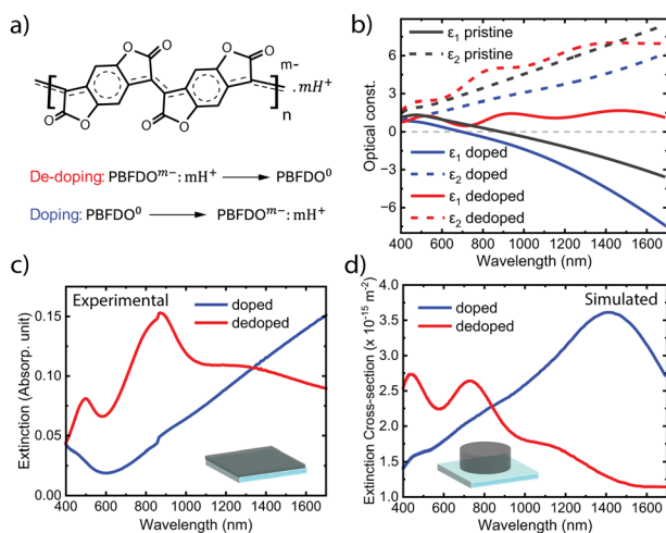
Fig. 1 (a) Chemical structure of n-doped PBFD0, and its doping/dedoping behaviour. (b) In-plane permittivity dispersion for PBFD0 thin films in the pristine state (black), after doping (blue) and de-doping (red). Full lines correspond to the real component ( \epsilon_1 ) and dashed lines correspond to the imaginary component ( \epsilon_2 ). (c) Experimental extinction spectra of a PBFD0 thin film (40 nm thickness) after chemical doping (blue) and dedoping (red). (d) Simulated extinction cross-section of a single PBFD0 nanodisk on glass in its doped (blue) and dedoped (red) states (80 nm diameter, 30 nm height).
