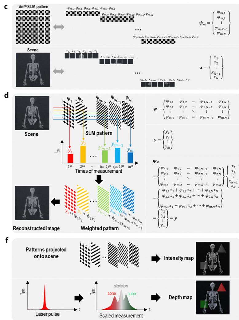
Fig. 1 Fundamentals of perovskite SPI. (a) Schematic of electromagnetic waves of different wavelength regions, covering gamma ray, X-ray, UV-Vis-NIR, and THz regions. (b) A typical SPI setup, usually termed as a “structured” setup. A light source (or arbitrary wavelengths) illuminates onto a scene object, and the reflected light is focused by an imaging lens onto a spatial light modulator (SLM), where a sequence of binary patterns is incorporated within the SLM to pattern the light to be further detected by the perovskite single pixel photodetector (PD). It should be noted that the perovskite PD simply records an overall photocurrent or photovoltage during each measurement. And for M measurements, a series of record electrical signals with M numbers are sequentially obtained by the PD. (c) The SLM can have different patterns for each measurement. For example, at the M th measurement, the SLM with N pixels can have a vector of \psi_m , which is mathematically expressed here. Similarly, when projected to this SLM, the light reflected from the scene object can be pixelated into N elements, with the scene being expressed by a vector of \mathbf{x} , which is mathematically expressed here as well. (d) Schematic showing how each measurement using differently patterned SLM to render different electrical signals (e.g., I_{ph} ) recorded by the detector, and how these two sets of matrices can be used to calculate the scene vector \mathbf{x} . (e) A deviated SPI setup with a time-of-flight attribute. By replacing the continuous wavelength light source with a pulse laser source, the pulse laser can incident to the SLM first for generating a transient light pattern onto the scene object (via a lens). The reflected pattern light (pulse laser light) off the object is detected by the single-pixel sensor. Due to the distance difference in the optical pathways, the temporal resolution corresponding to the 3D geometry of the scene object is encoded within the electrical signal of the photodetector, providing a measure of the distance the light has traveled thereby revealing the depth of the scene. (f) As with the structured detection approach, the sequence of projected patterns and their corresponding intensity measurements enable image reconstruction. When using a pulsed laser, the time-of-flight information from the broadened backscattered light pulse additionally allows for the creation of a depth map of the scene. Fig. 1b–f are adapted with permission from ref. 31, copyright © 2020 Optical Society of America under the terms of the OSA Open Access Publishing Agreement.
